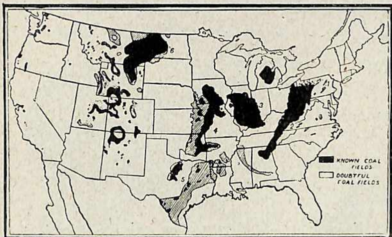
COAL deposits in Britain and the United States. The iron ore deposits in the U.S.A. are mainly located adjacent to the Eastern coal fields.
